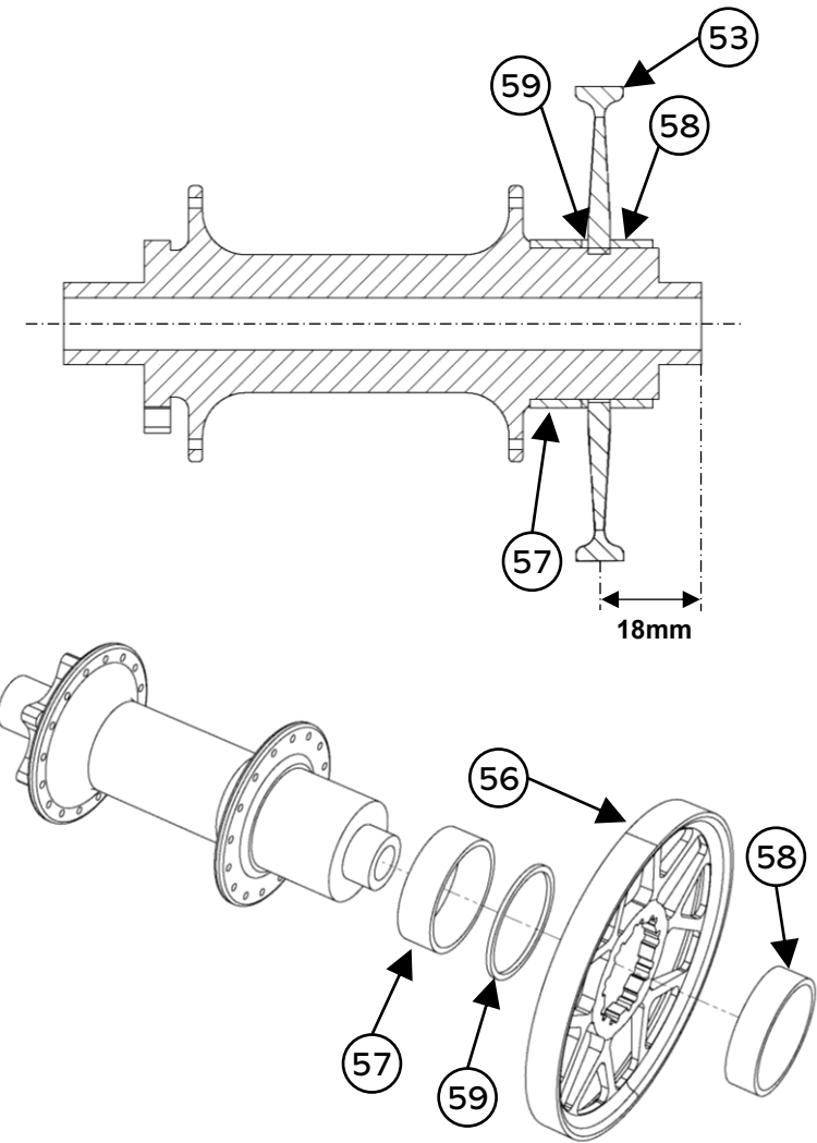
Clutch 160.7
