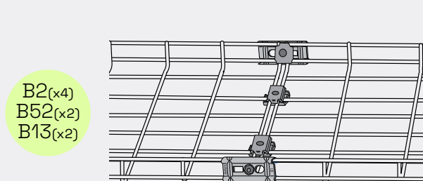
Splicing mesh tray Width 422 mm
