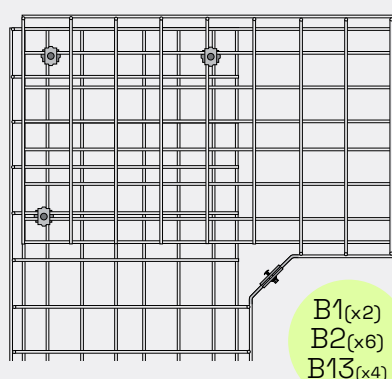
Rounded 90° elbow
