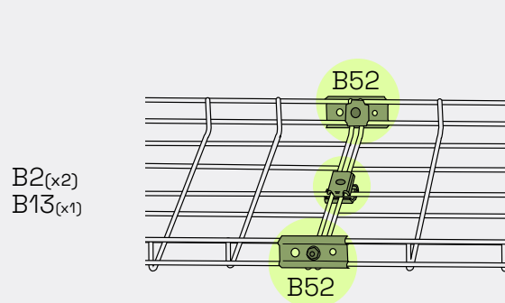
Splicing mesh tray Width 320 mm
