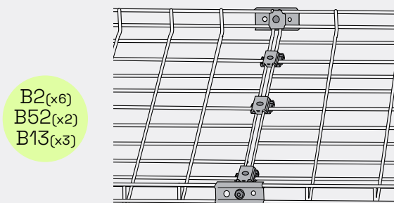
Vertical riser
