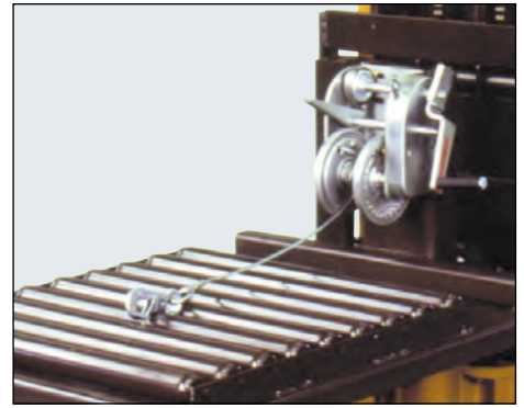
Die Puller Front-load roller platform, 1000 lb. capacity (with proper straddles), complete with winch. Secures to rigid or adjustable forks.
