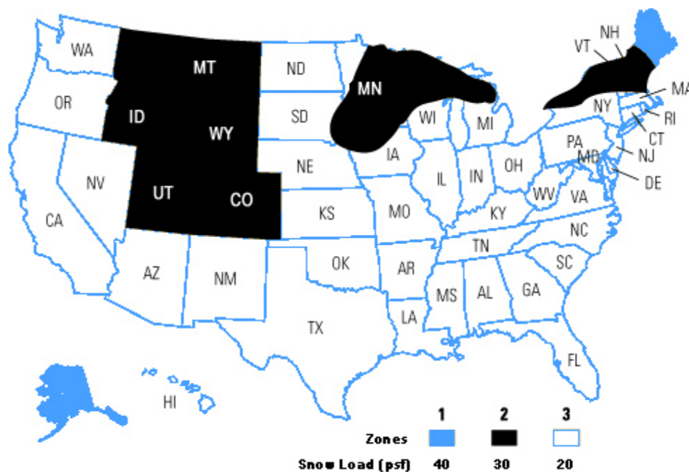
Figure 6. Roof (snow) load map
