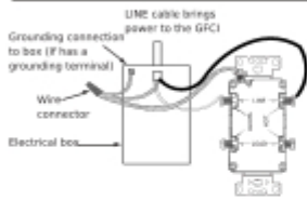
A: One cable (2 or 3 wires) entering the box
