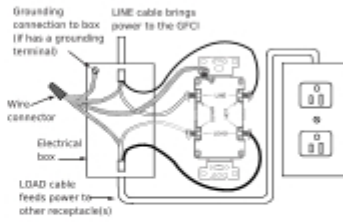
OR B: Two cables (4 to 6 wires) entering the box
