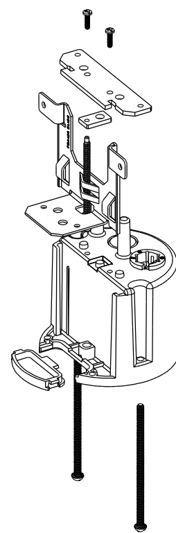
ISOMETRIC ASSEMBLY VIEWS
