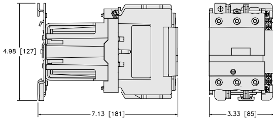
CONTACTOR WITH DC COIL
