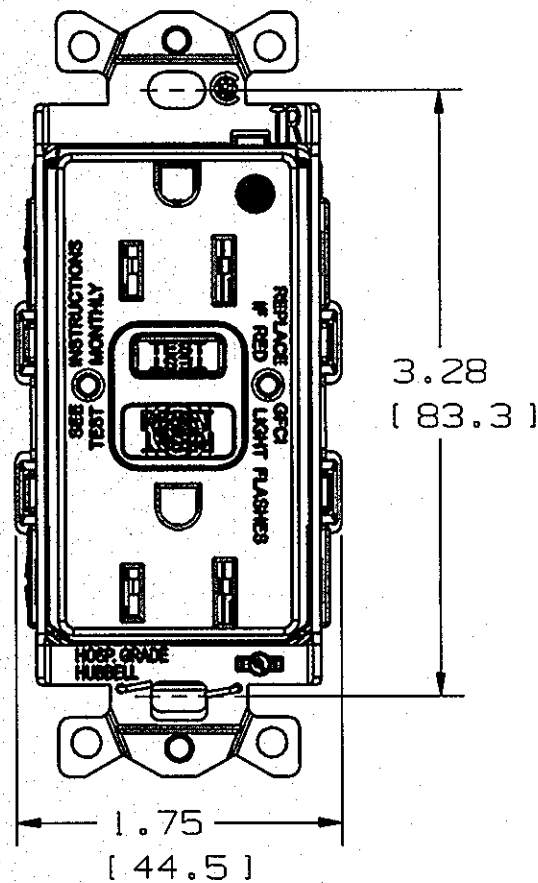
15A DEVICE
