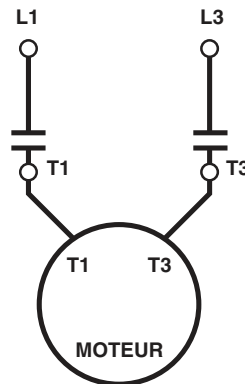
1 PHASE
