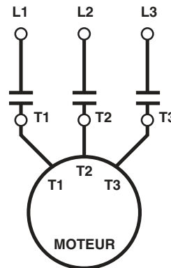
3 PHASE
