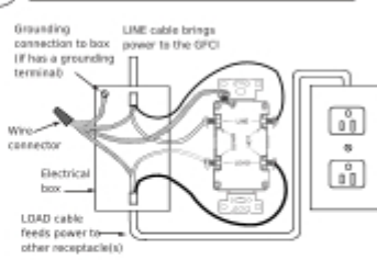
OR B: Two cables (4 to 6 wires) entering the box
